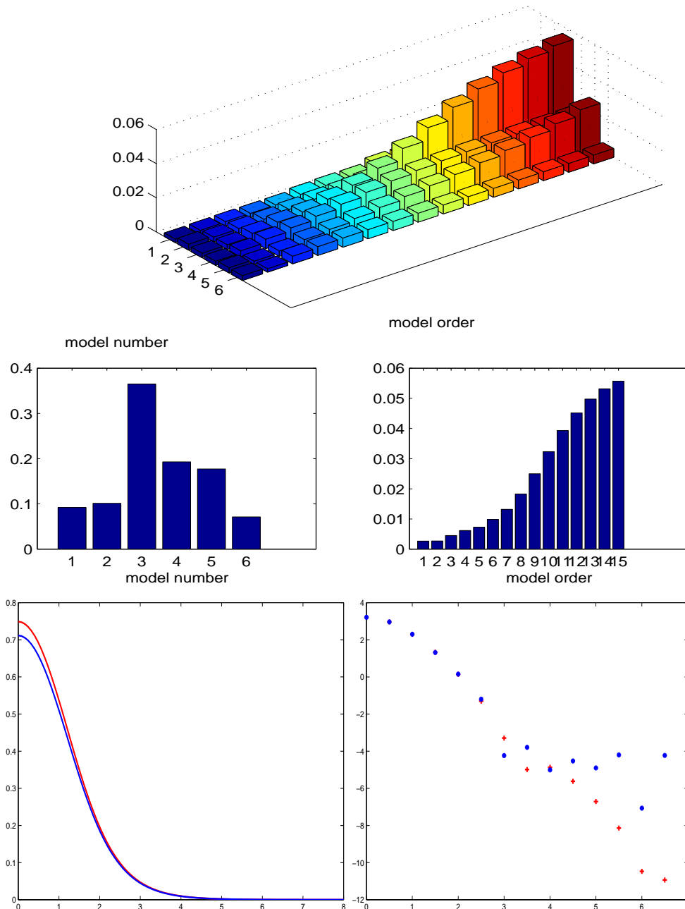
Fig. 7: a) p(k, l | \mathbf{y}) b) p(k | \mathbf{y}) c) p(k | \mathbf{y}, \hat{l}) d) \rho(r) and \hat{\rho}(r) e) F(q_i) and \hat{F}(q_i) .
